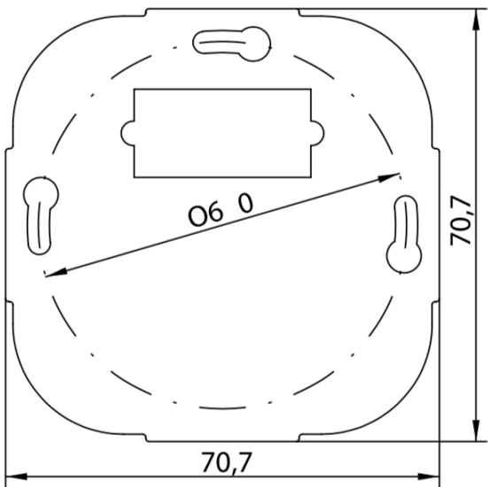
Mounting:
